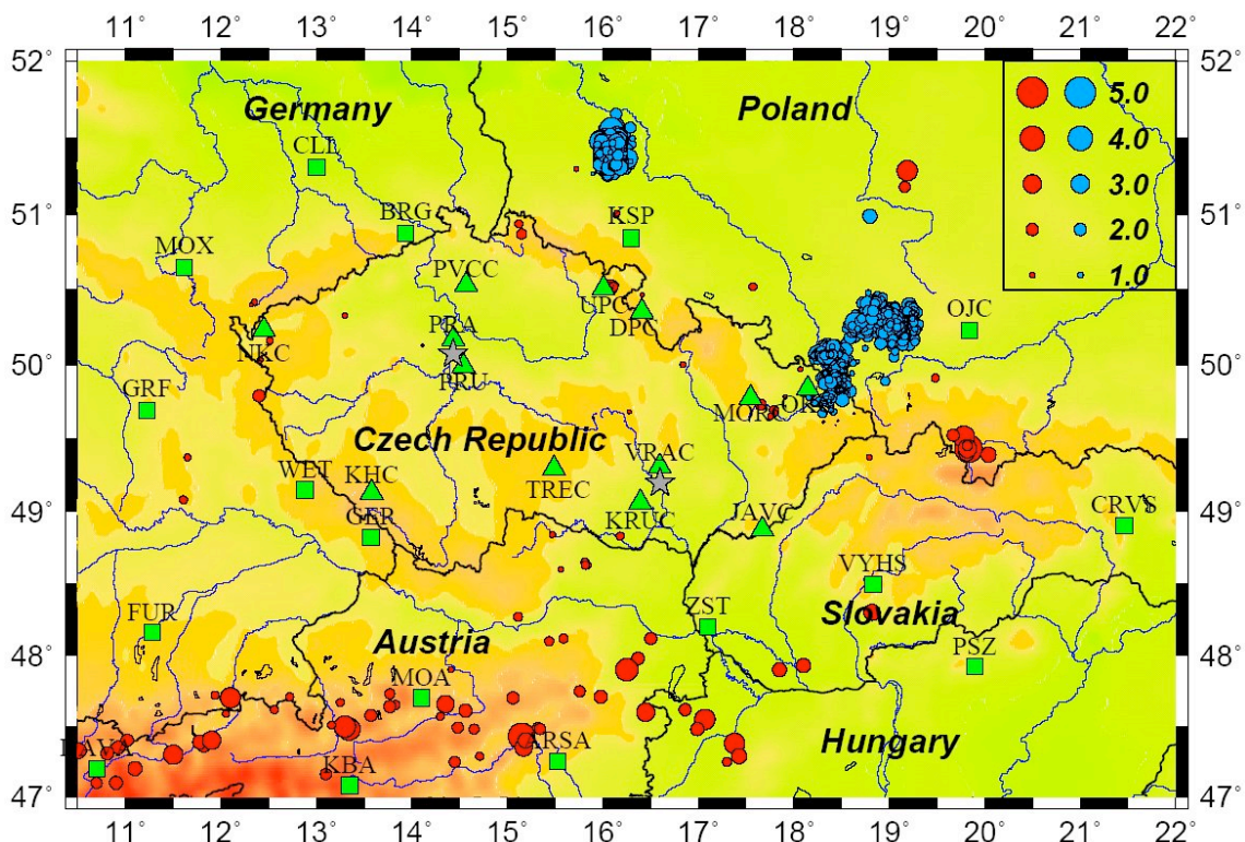
Fig. 1. Permanent seismological stations in Czech Republic in 2005 (green triangles - operational stations; squares – stations in neighbouring countries; stars – GI-ASCR and IPE-MUB data centers; red circles – epicentres of earthquakes in 2004, blue circles - mining-induced seismic events in 2004.
